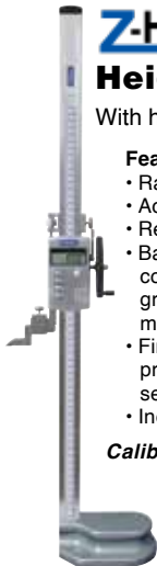
24" Height Gage shown
